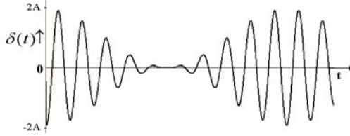
Fig. 19. Plot of \delta(t) function
