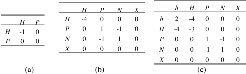
Fig. 20. Interaction potential matrixes of (a) HP (b) HPNX [89] and (c) hHPNX model. Negative entry indicates reward for being topological neighbors (TN) in the lattice model, whereas interaction for TN with positive value represents a penalty, ‘0’ indicates neutral (i.e., no) interaction.
